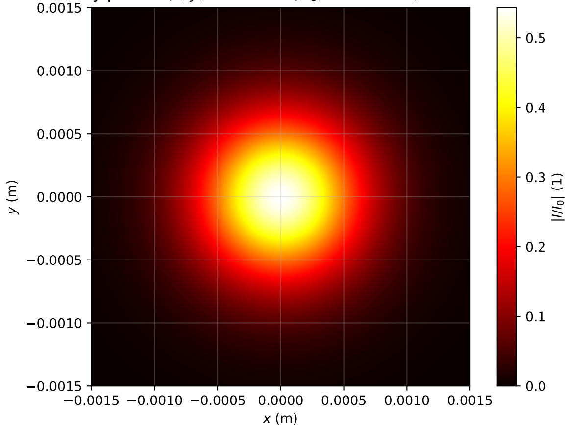
Intensity profile I(x, y, z = 3.105m)/I_0 , P_{in}=0.5P_{cr} , artificial time
